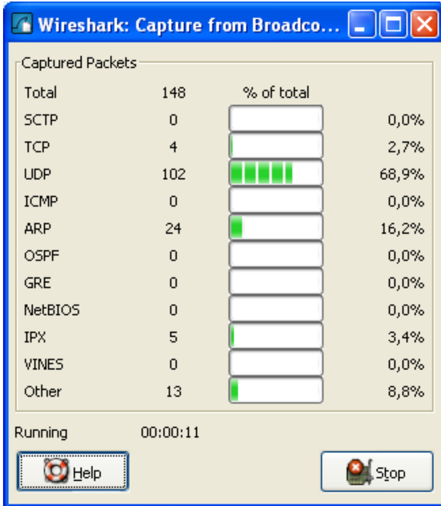
Figure 4.5. The "Capture Info" dialog box
