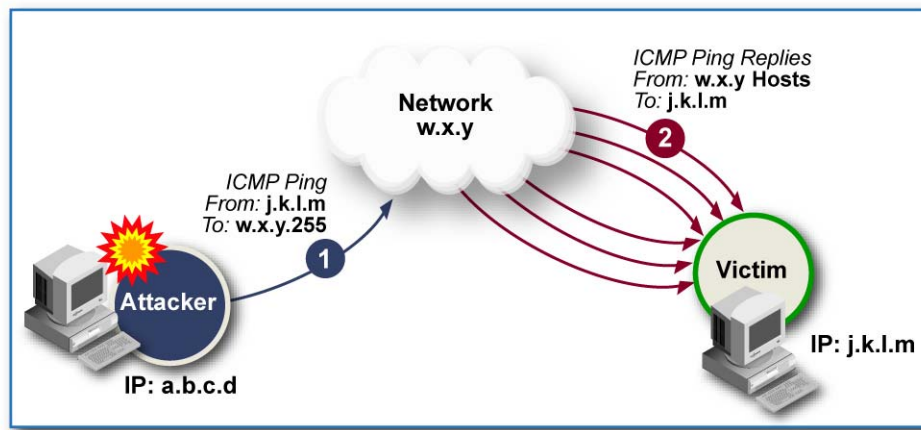
Figure 4-2. Amplifier Attack
