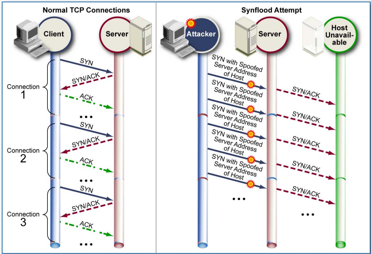
Figure 4-4. Synflood Attack
